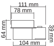
Cassaforma laterale Lateral formwork
