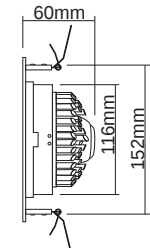
Vista laterale Side view
