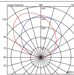
Emissione a fascio diffuso / Diffuse beam
