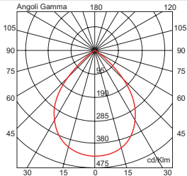
Emissione a fascio diffuso / Diffuse beam
