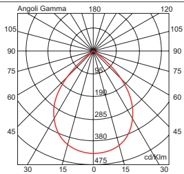
Emissione a fascio diffuso / Diffuse beam
