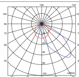
Emissione asimmetrica / Asymmetric beam
